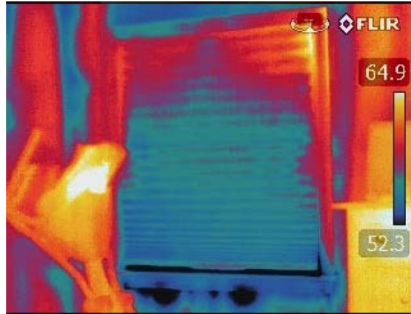
Figure 21. House 3 interior infrared image of bedroom window
