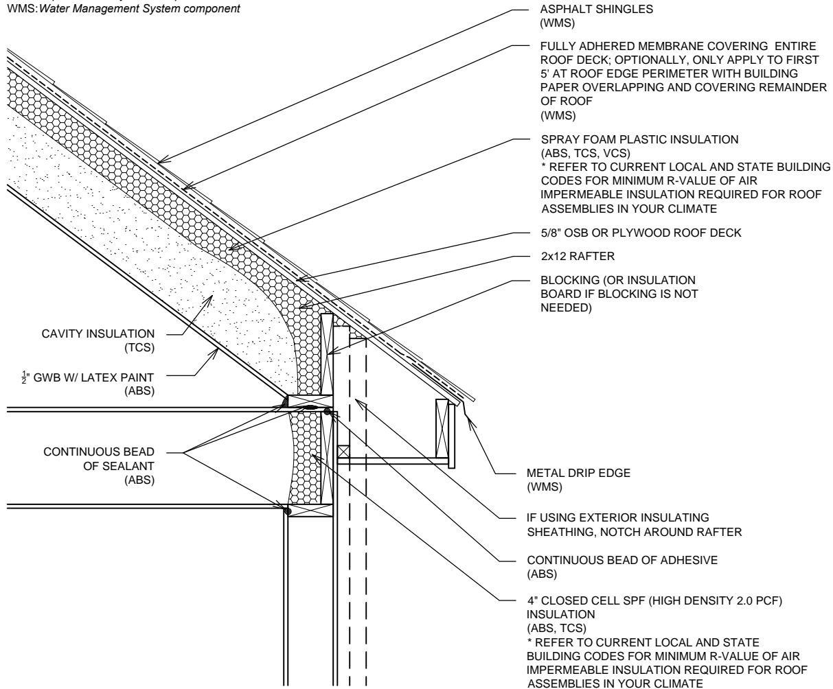
UNVENTED ATTIC 2x12 RAFTER - INSULATION BELOW ROOF DECK IN RAFTER CAVITY
