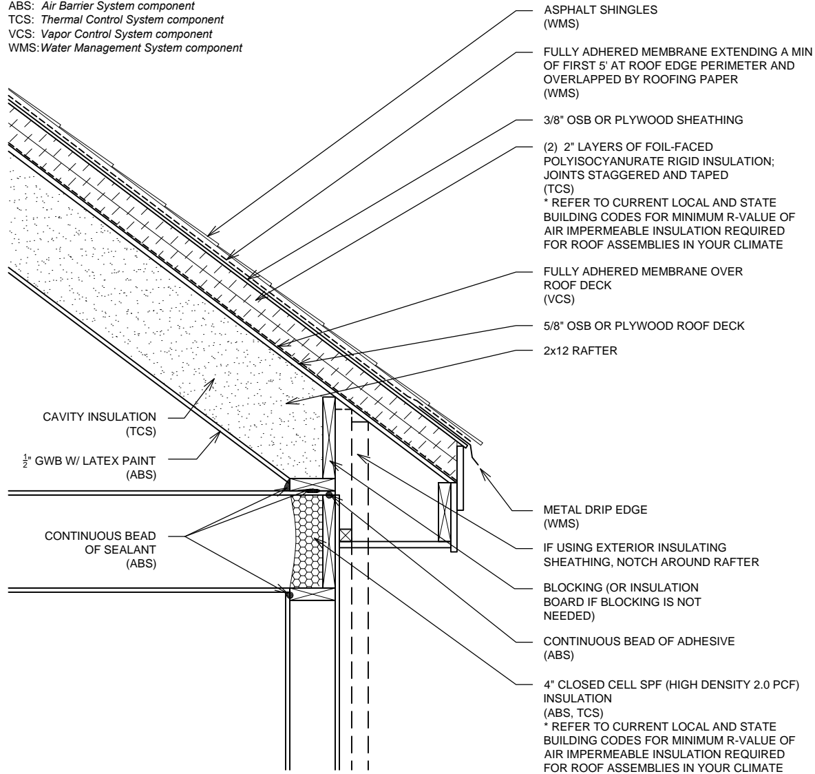
UNVENTED ATTIC 2x12 RAFTER - INSULATION ABOVE ROOF DECK AND IN RAFTER CAVITY
