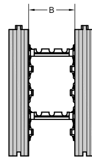
6" CONNECTOR
