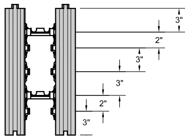
4" CONNECTOR
